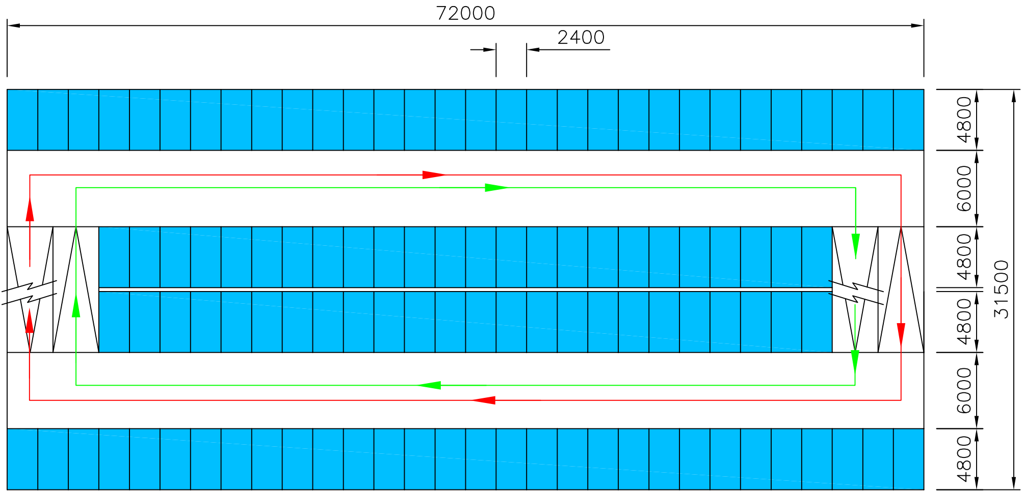
Split Level Parking Deck with Internal Ramps
