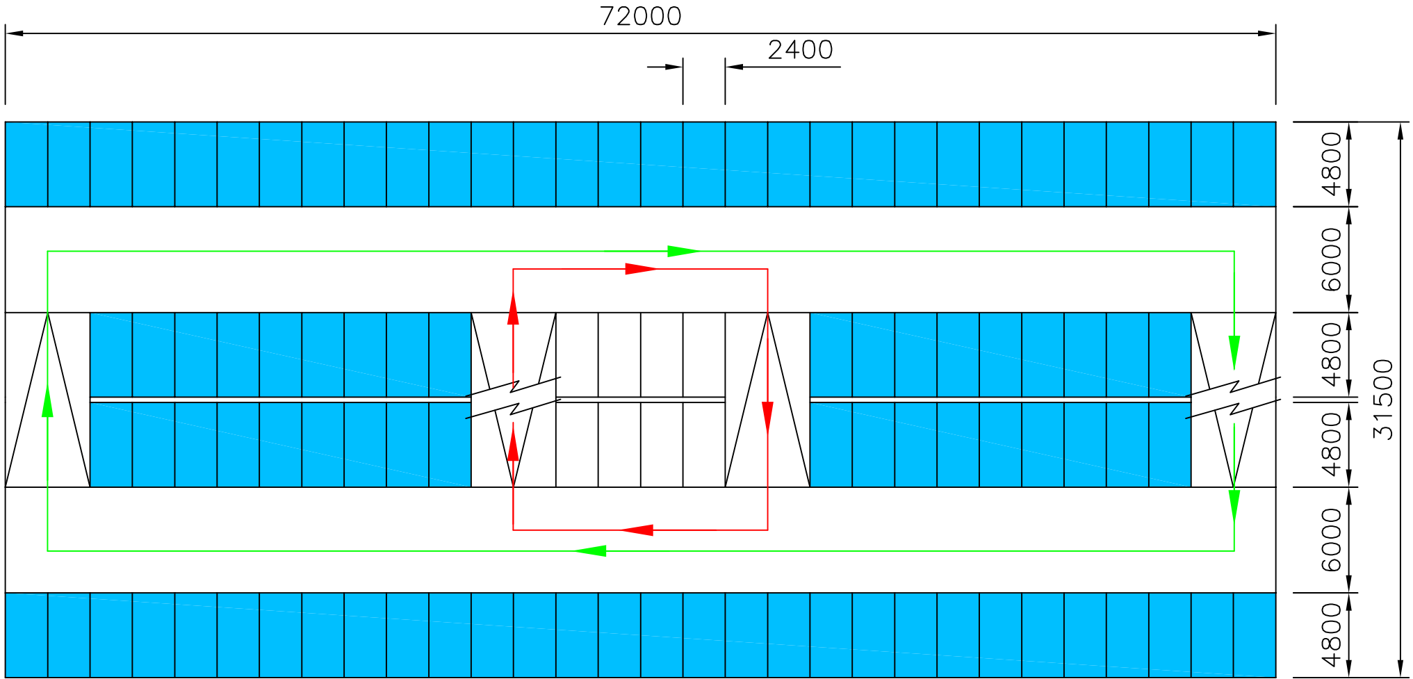
Split Level Parking Deck with Internal Ramps (shortened exit route)
