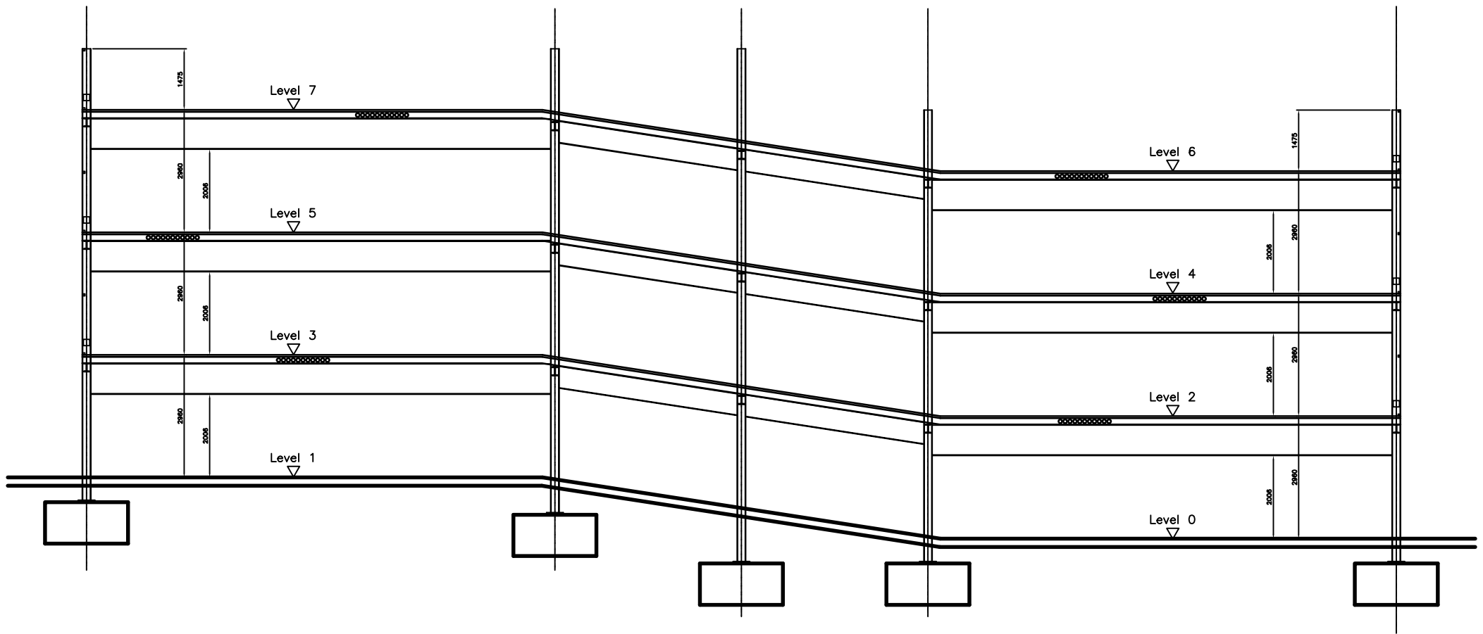
Typical Section - Split Level
